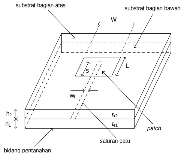
Gambar 1. Geometri Pencatutan electromagnetically coupled [satu baris kosong]
